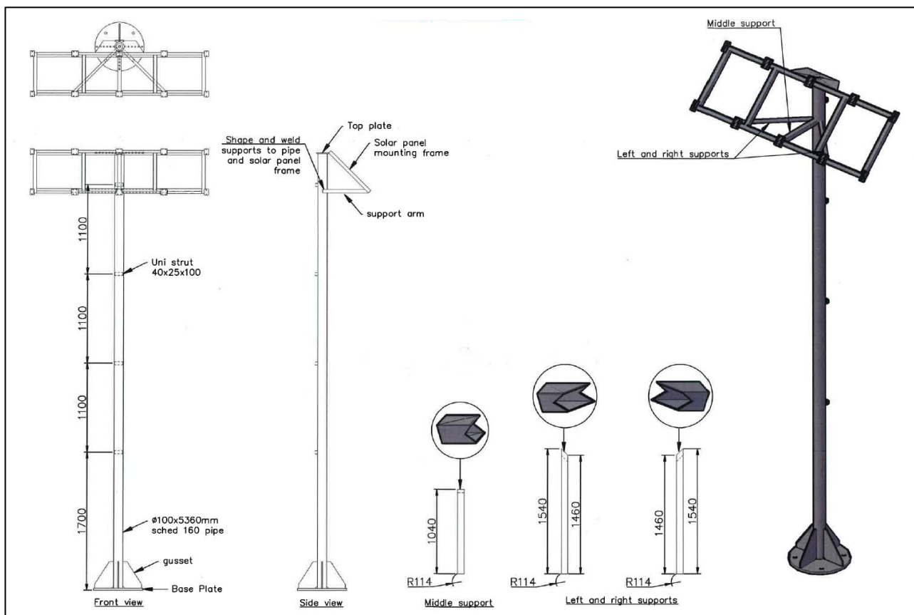
Figure 3 – Typical Fixed Pole Solar Installation
